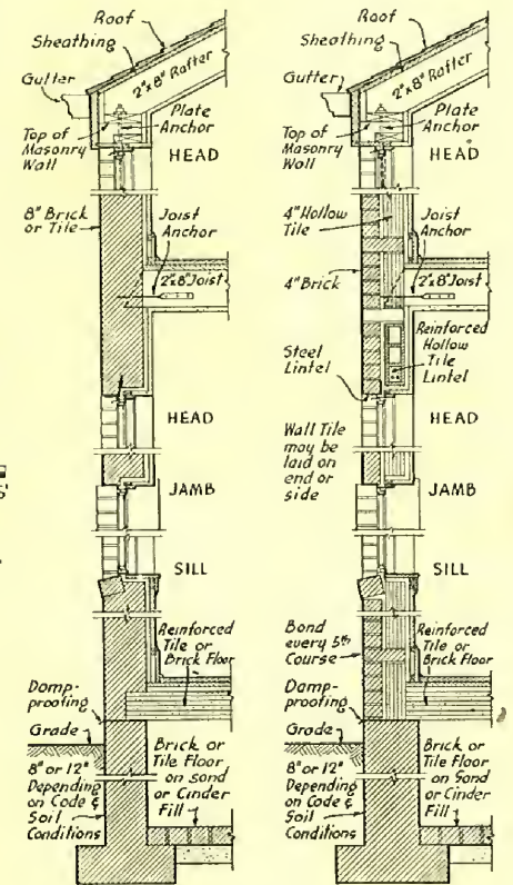
Wall Sections
